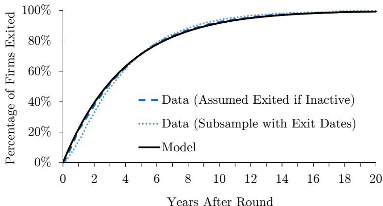
Fig. 2. Time to Exit Dispersion in VentureSource and Model. This figure reports the percentage of firms that have exited at different times after a financing round. Our model (solid line) has firms exit at an exponential rate of \lambda = 0.25 . This is compared to the time to exit for fourth or later VC financing rounds in VentureSource data from mid-1992 to mid-2015. We look at both firms with reported exits (dotted line) and firms that either reported an exit or were inactive for three years (dashed line). We assume the inactive firms failed uniformly in the year after their last reported financing round.
